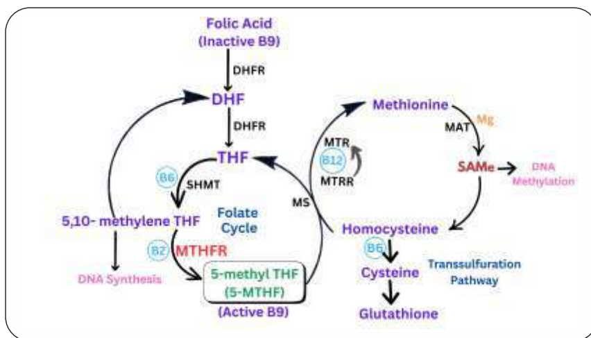
Figure 2: Folate Cycle
